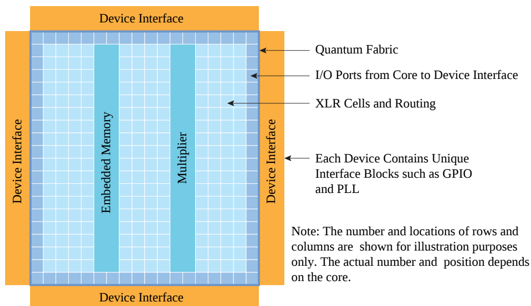
Figure 1: T55 FPGA Block Diagram
