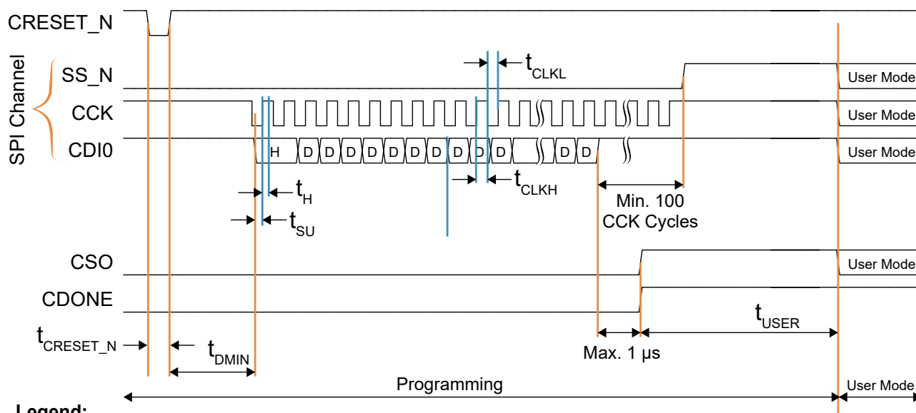
Figure 33: SPI Passive Mode (x1) Timing Sequence
