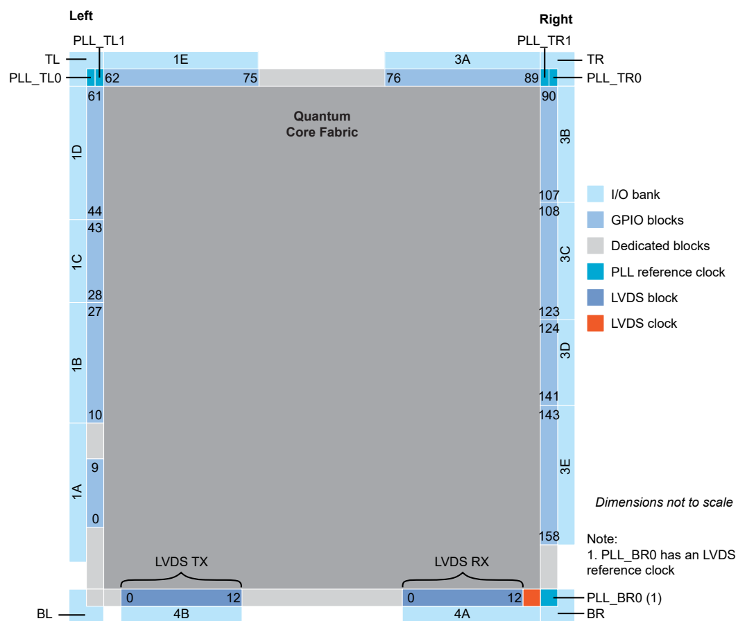
Figure 35: Floorplan Diagram for Q100F3 Packages
