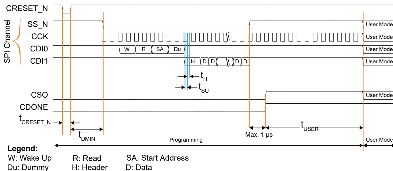
Figure 32: SPI Active Mode (x1) Timing Sequence
