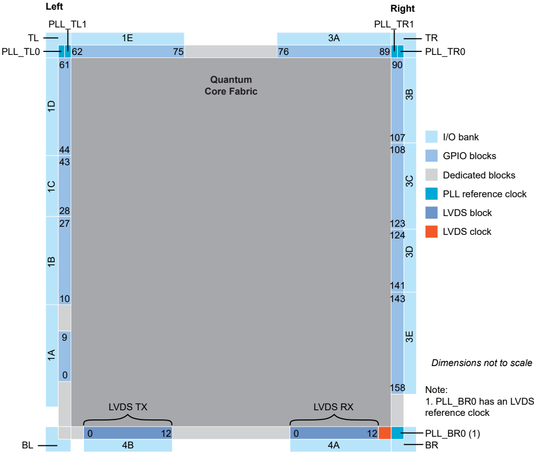
Figure 37: Floorplan Diagram for F256 Packages
