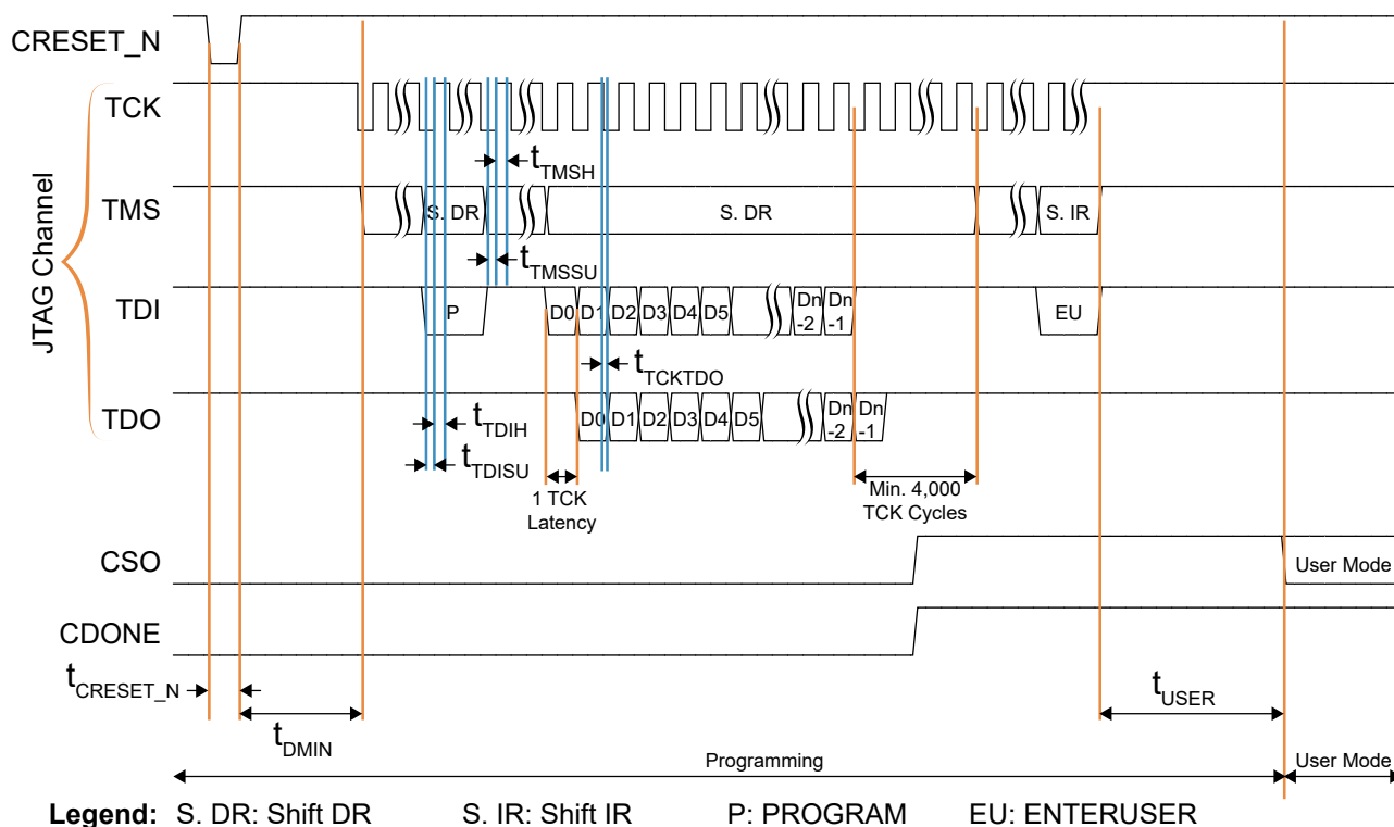
Figure 34: JTAG Programming Waveform
