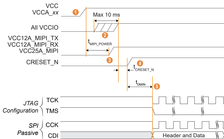
Figure 26: Trion® FPGAs Power Up Sequence
