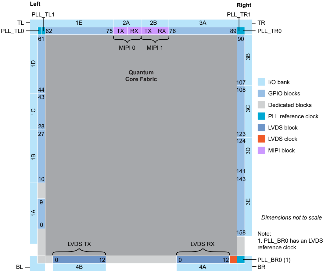
Figure 36: Floorplan Diagram for F169 Packages (with MIPI)
