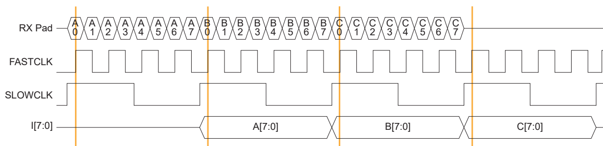
Figure 17: LVDS RX Timing Example Serialization Width of 8
