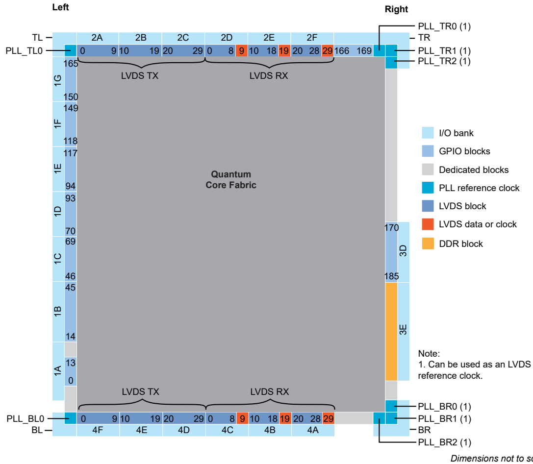
Figure 37: Floorplan Diagram for F484 Packages (with DDR)
