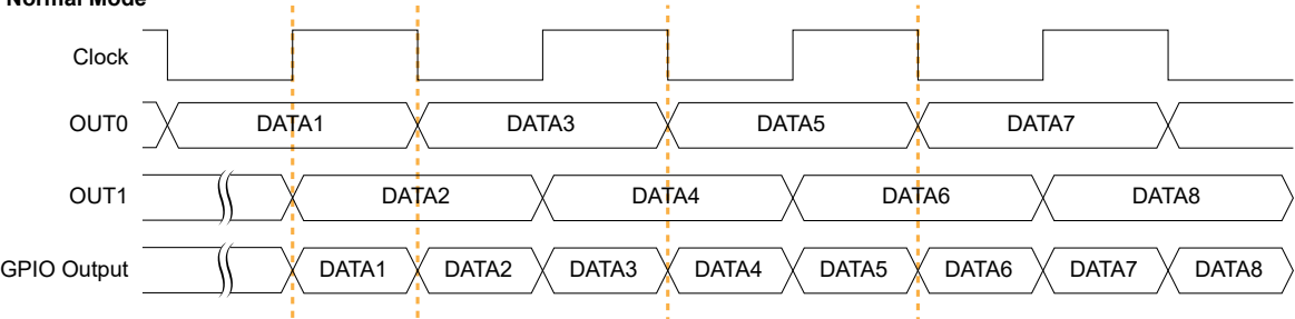
Figure 9: DDIO Output Timing Waveform
