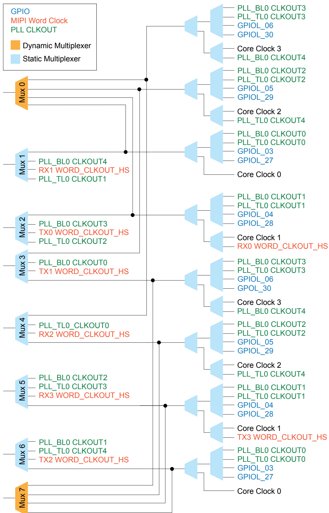
10: Clock Sources that Drive the Multiplexers: Left
