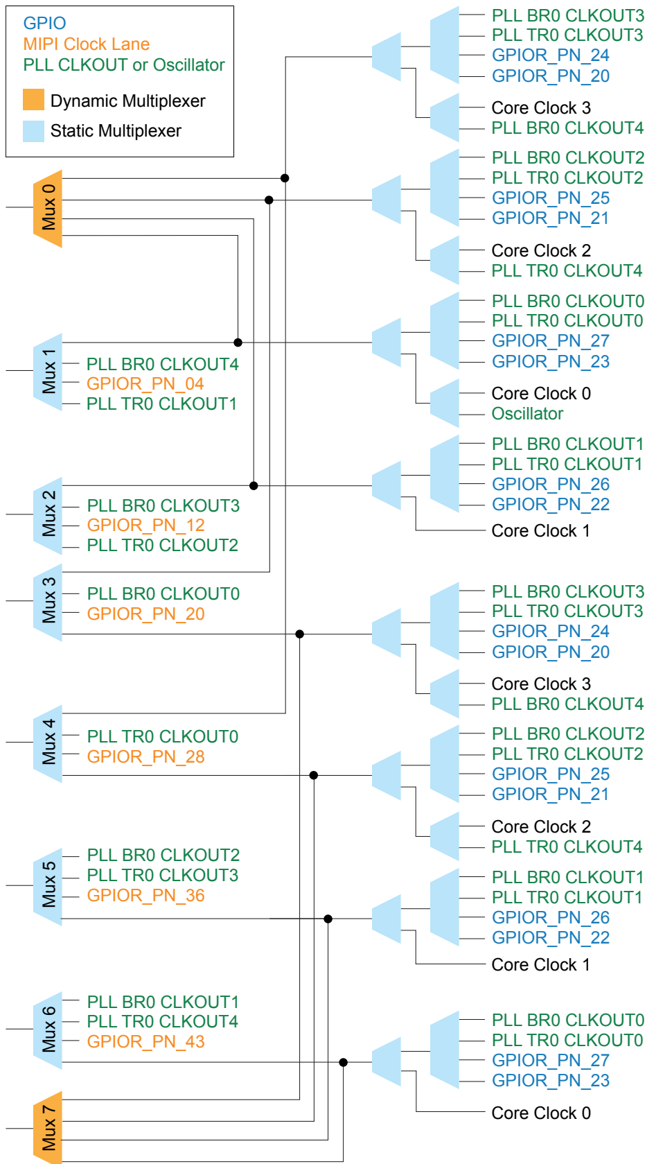
图 11: Clock Sources that Drive the Multiplexers: Right
