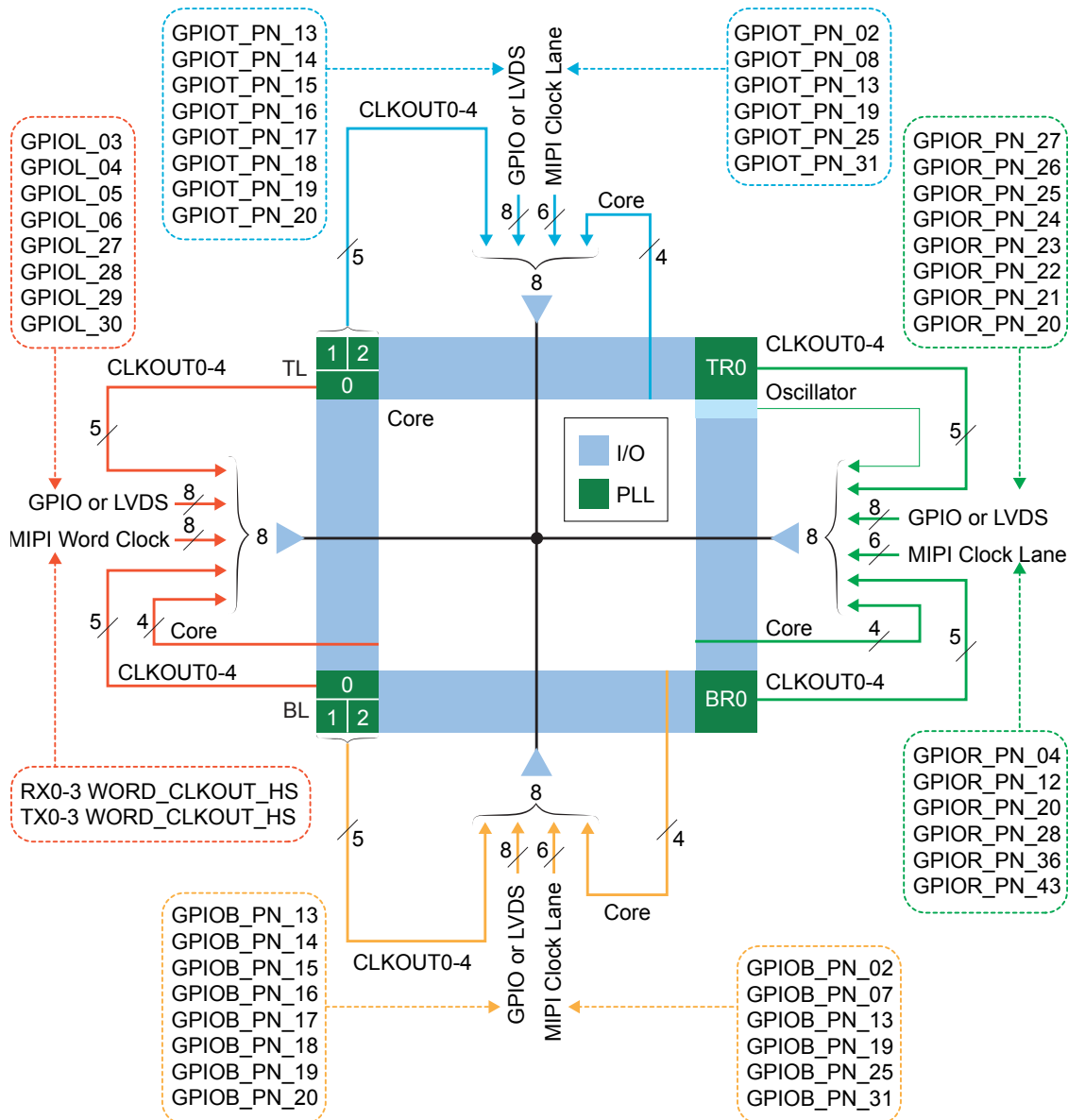
图 7: Clock Sources that Drive the Global Network
