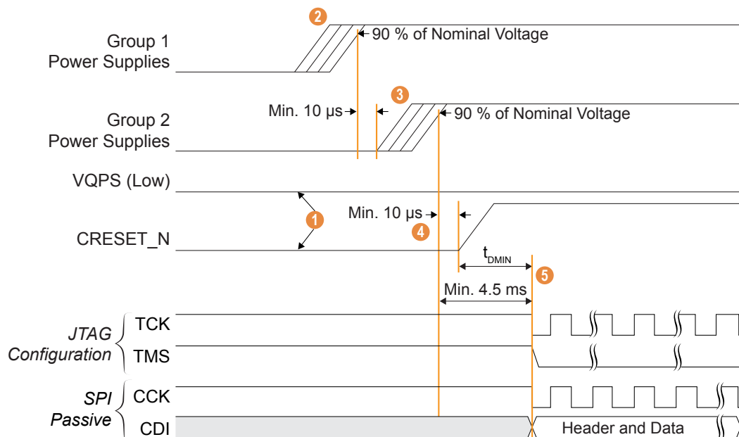
图 46: Power-Up Sequence
