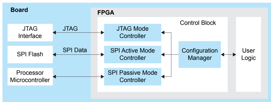
图 47: High-Level Configuration Options
