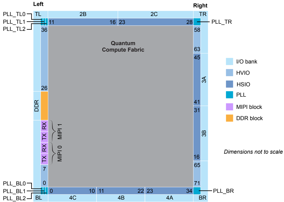
图 52: Floorplan Diagram for J361 Packages
