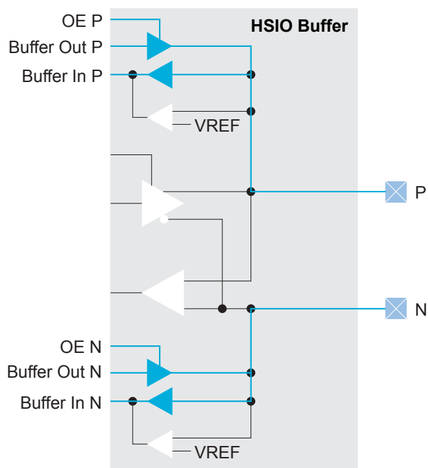
21: I/O Buffer Path for LVC MOS
