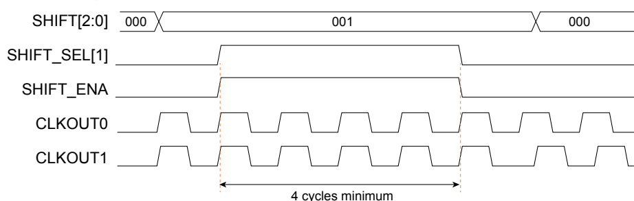
图 41: Consecutive Dynamic Phase Shift Waveform Example for CLKOUT1
