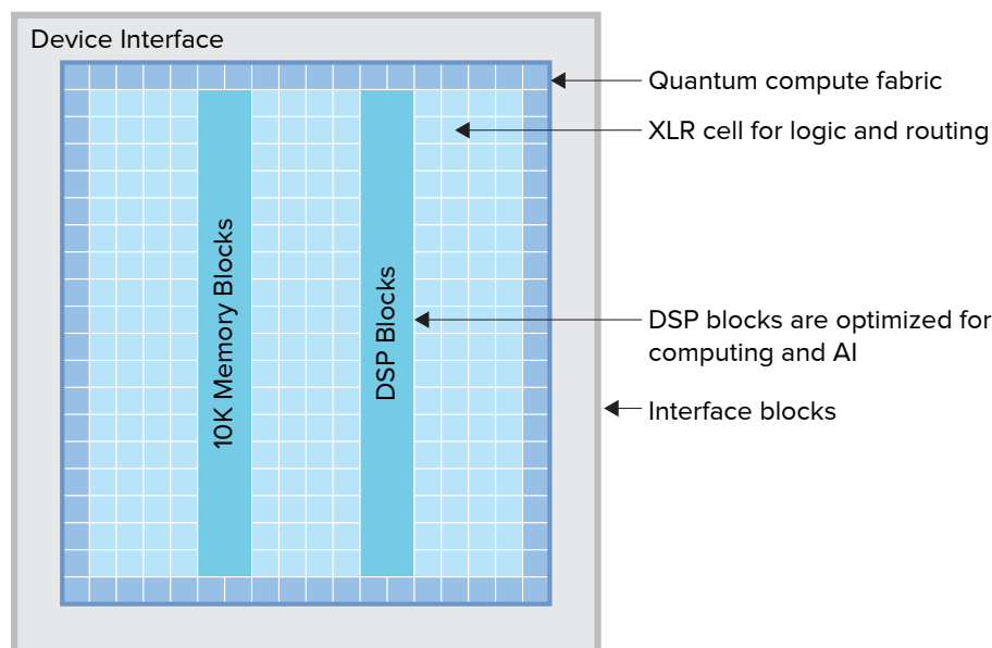
图 1: Ti120 FPGA Block Diagram
