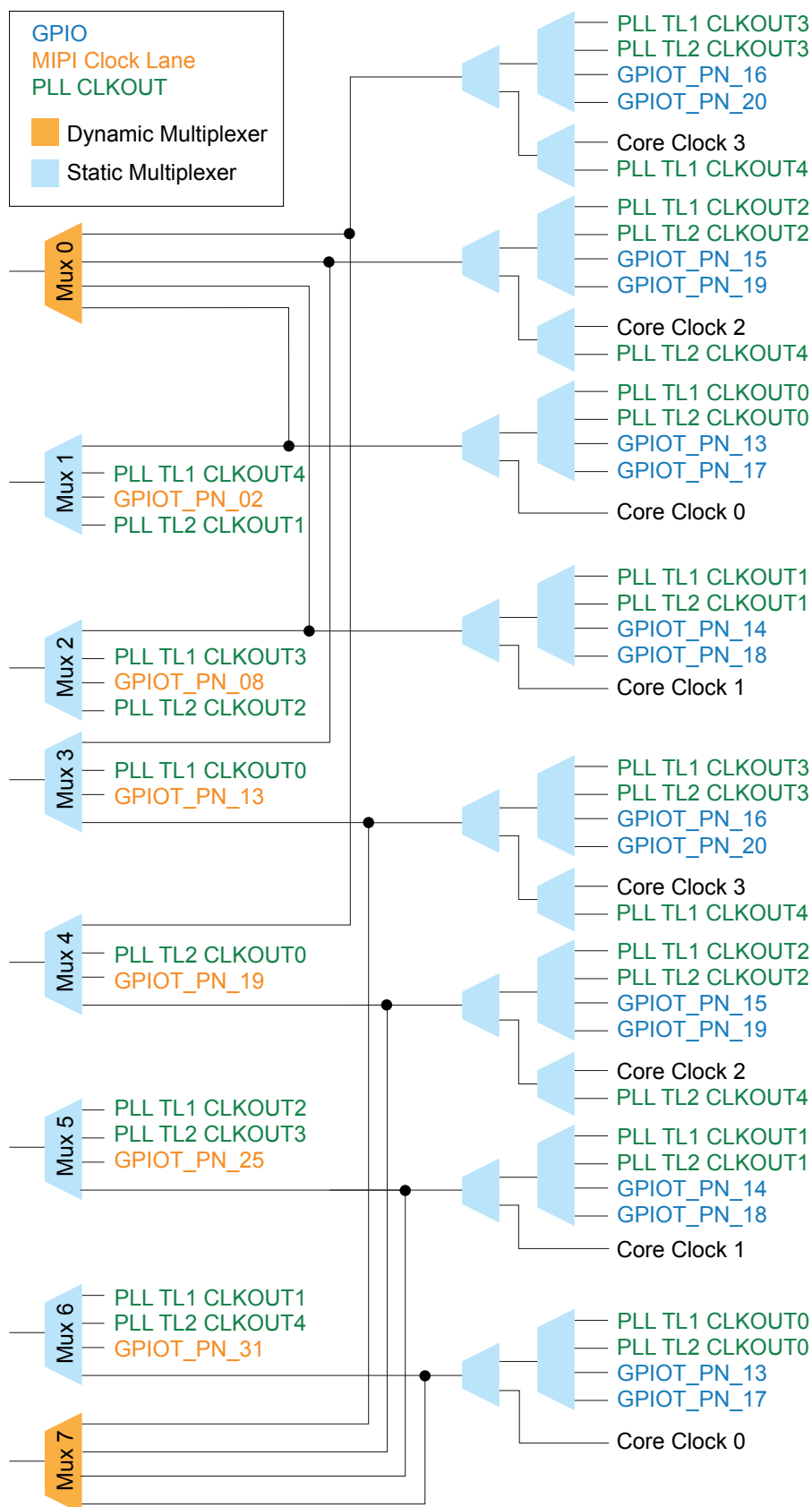
图 8: Clock Sources that Drive the Multiplexers: Top
