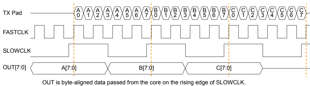
图 27: LVDS Timing Example Serialization Width of 8 (Half Rate)
