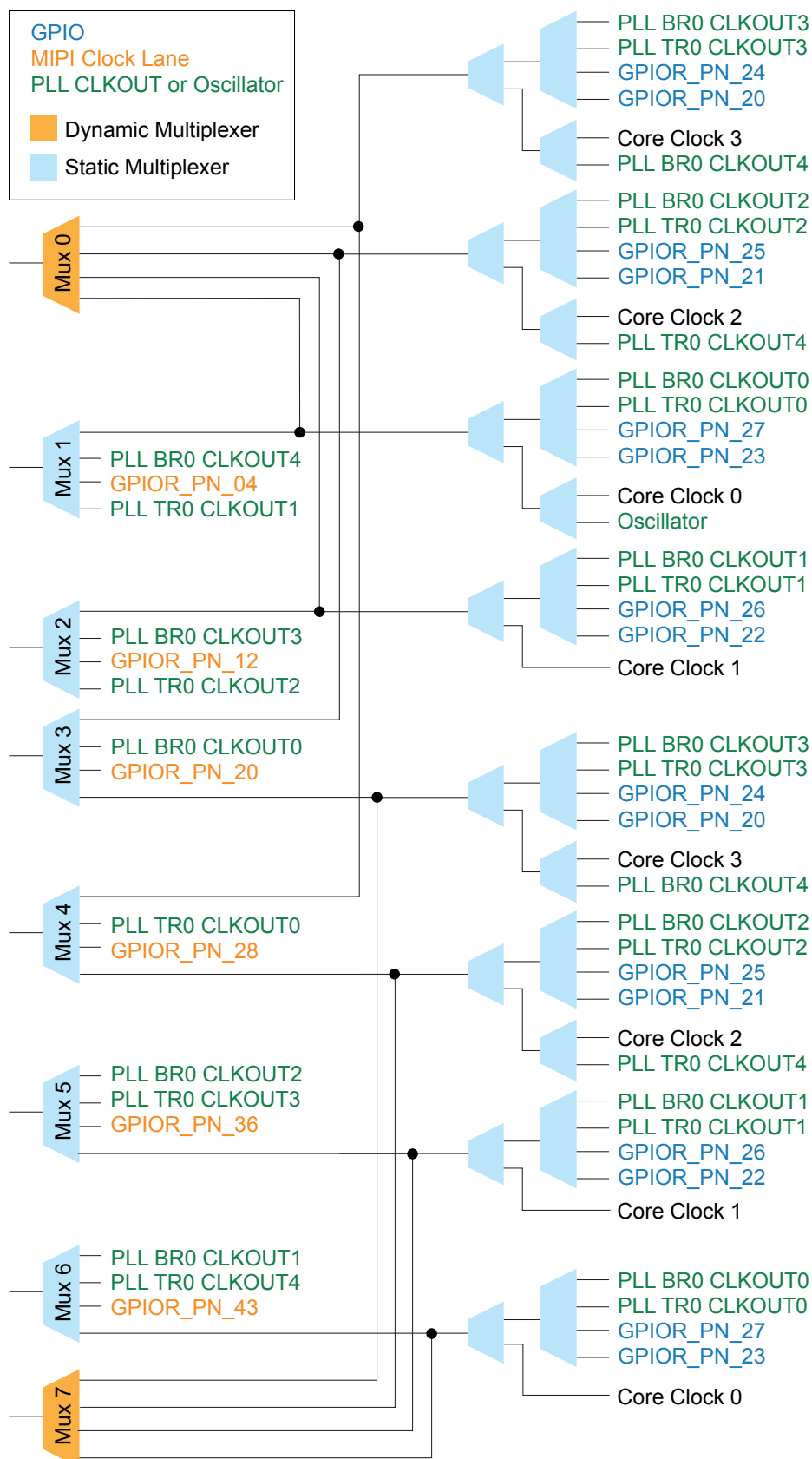
图 11: Clock Sources that Drive the Multiplexers: Right
