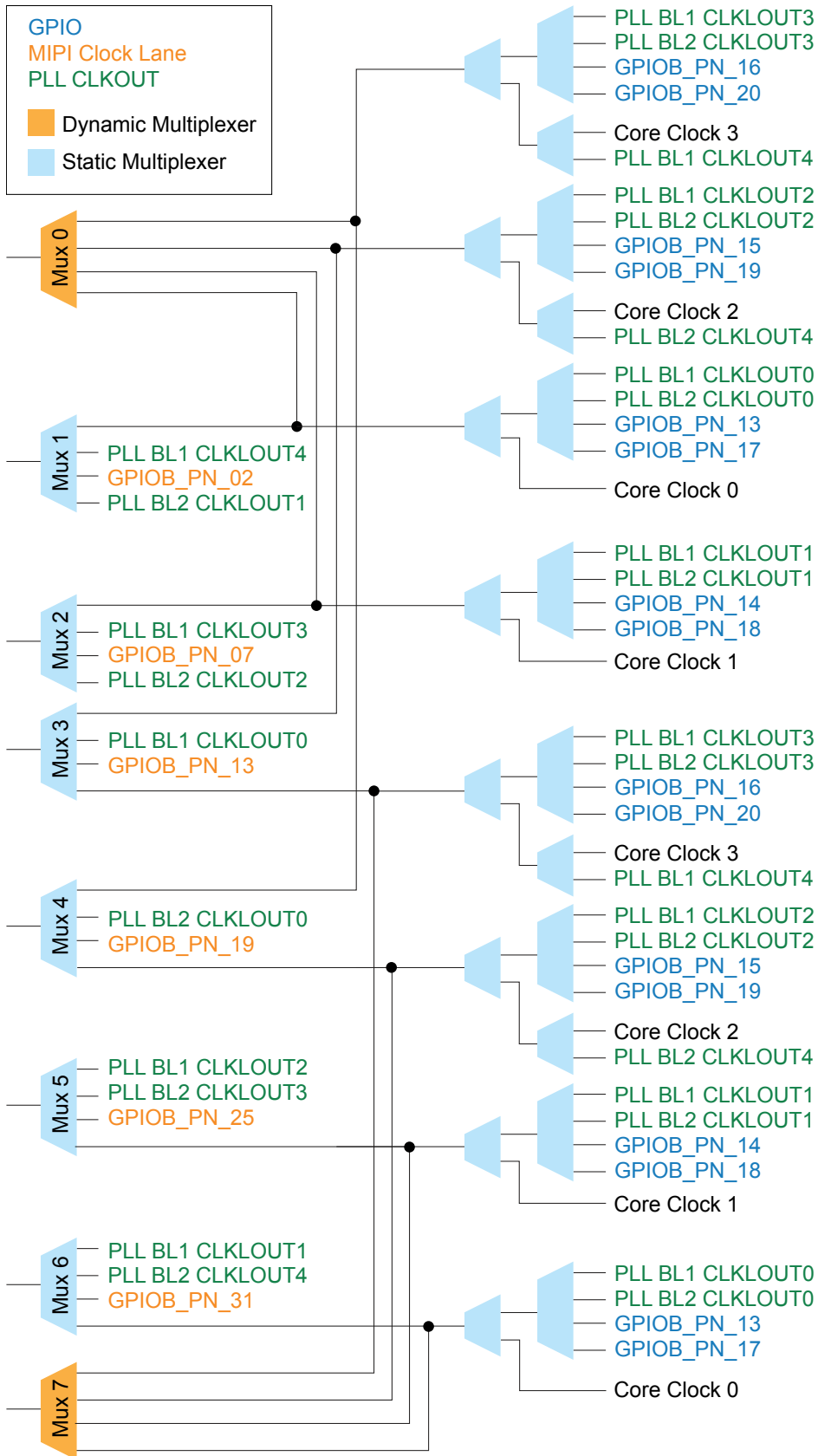
图 9: Clock Sources that Drive the Multiplexers: Bottom
