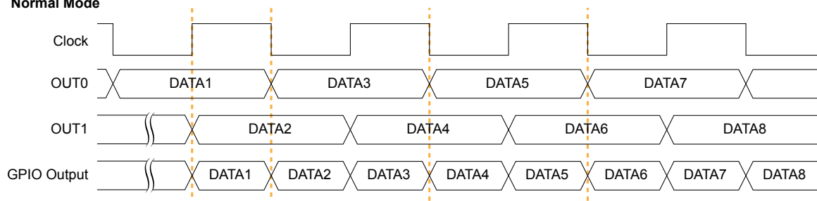
图 9: DDIO Output Timing Waveform
