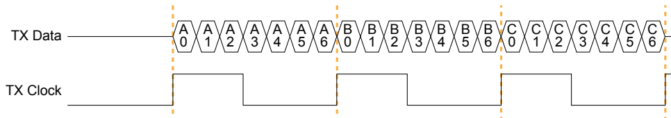
图 18: LVDS Timing Data and Clock Relationship Width of 7 (Parallel Clock Division=1)
