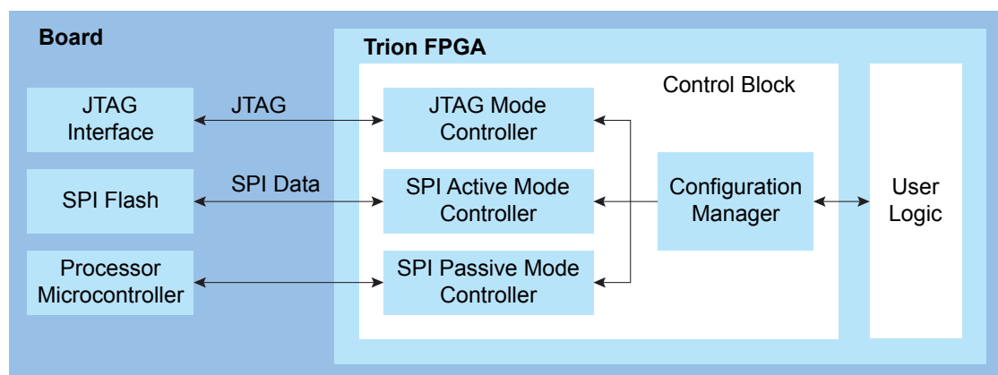
图 22: High-Level Configuration Options
