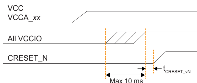
图 21: Trion® FPGAs Power Up Sequence
