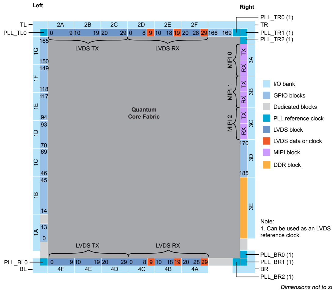
图 38: Floorplan Diagram for BGA576 Packages (with DDR and MIPI)
