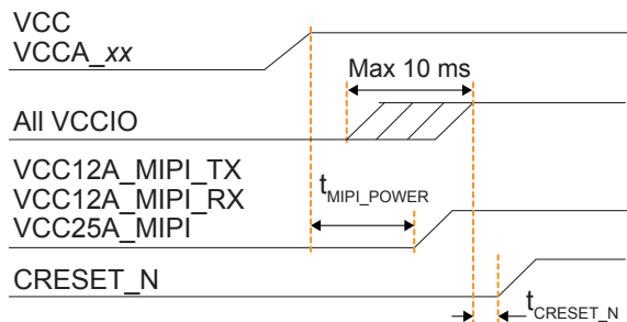
图 27: Trion® FPGAs Power Up Sequence
