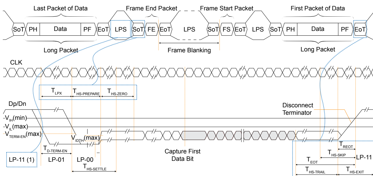
23: High-Speed Data Transmission in Bursts Waveform
