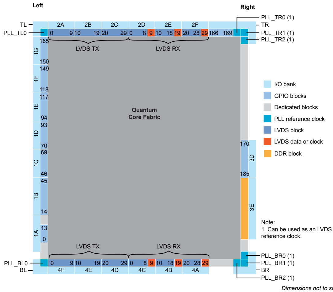
图 37: Floorplan Diagram for BGA484 Packages (with DDR)
