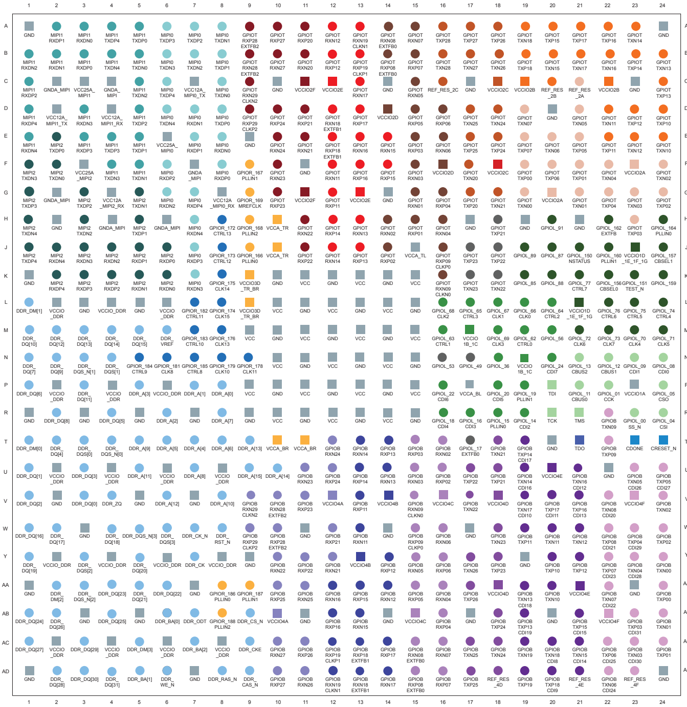
Figure 40: 576-Ball FBGA I/O Bank Diagram
