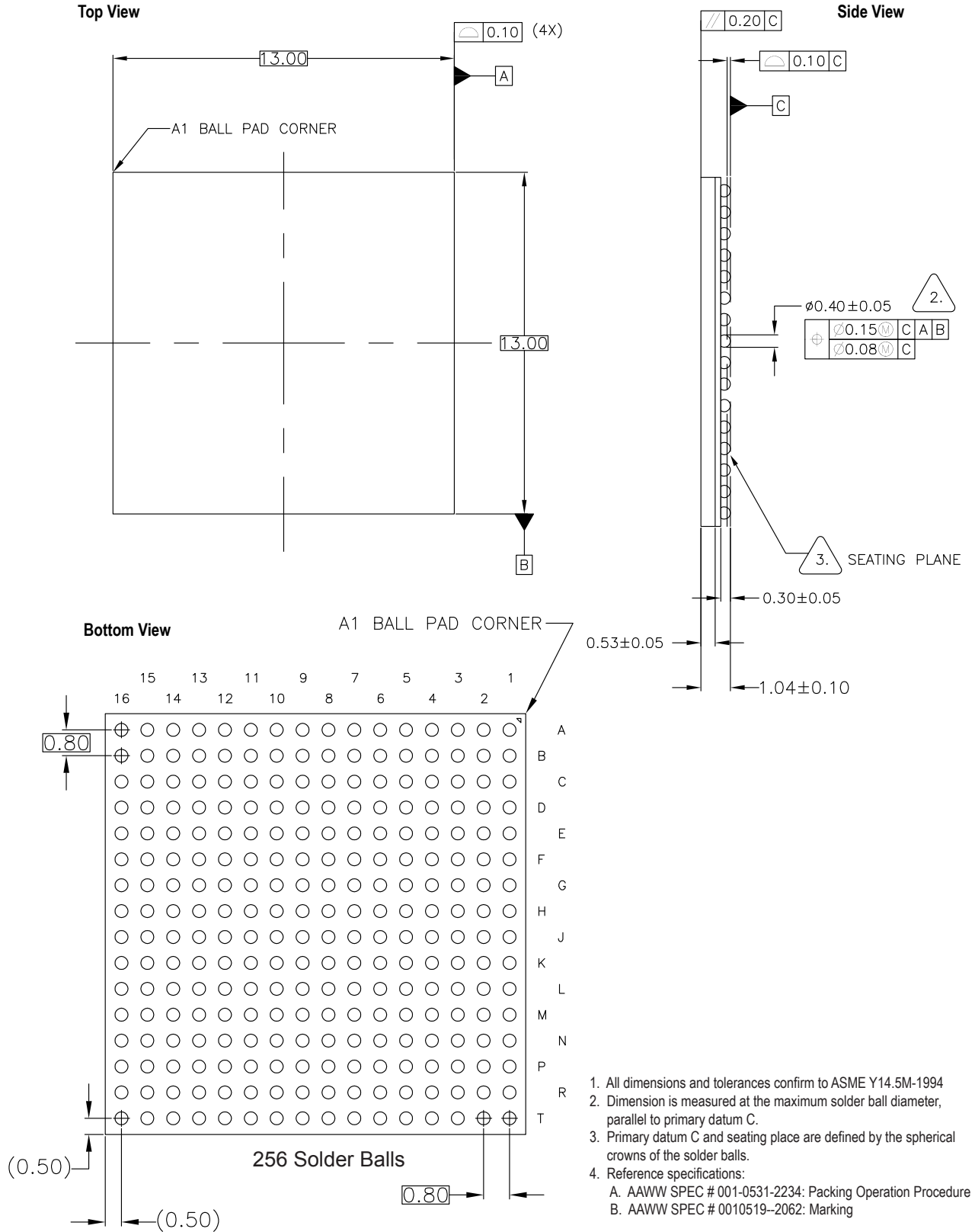
Figure 24: 256-Ball FBGA Package Outline
