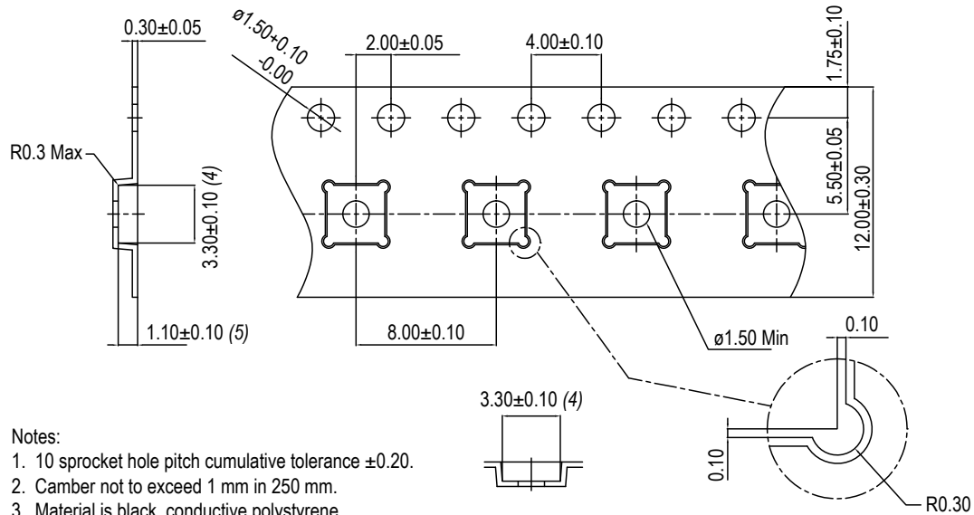
Figure 51: Tape Outline (BGA49 Packages)
