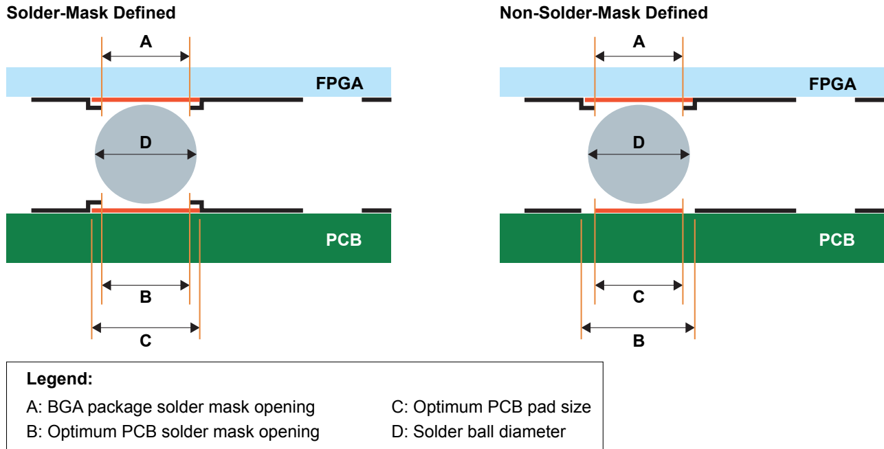
Figure 44: SMD and Non-SMD Pad Specification
