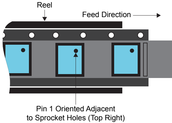
Figure 54: Tape Outline (WLCSP80 Packages)
