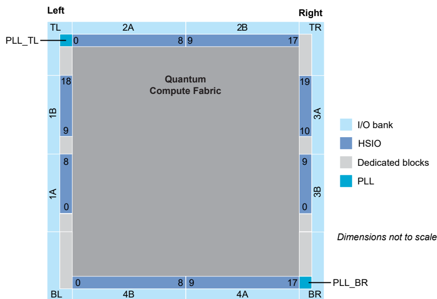
Figure 44: Floorplan Diagram for W64 Packages
