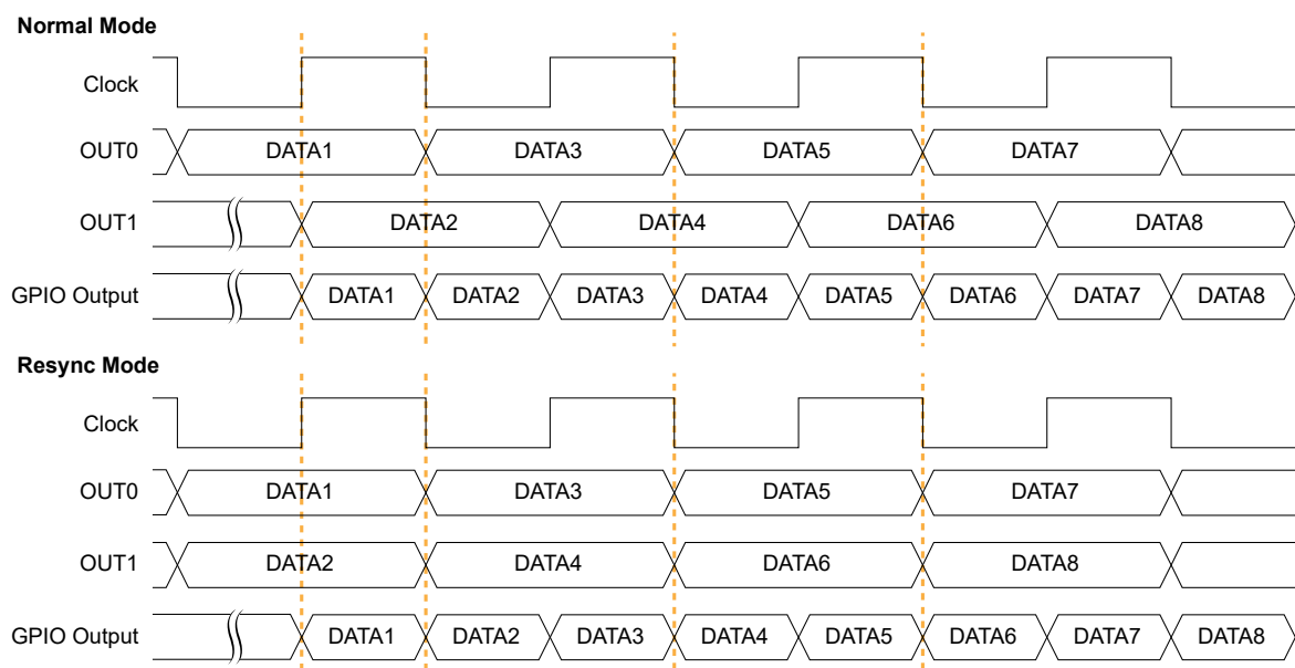
Figure 17: DDIO Output Timing Waveform
