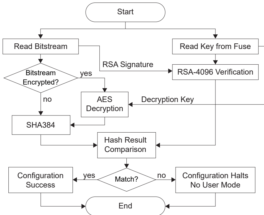
Figure 38: Security Flow
