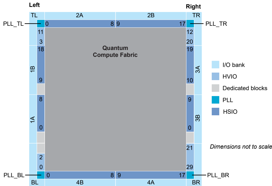
Figure 44: Floorplan Diagram for Ti35
