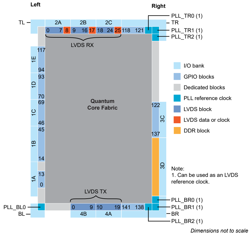
Figure 34: Floorplan Diagram for BGA400 Packages (with DDR)
