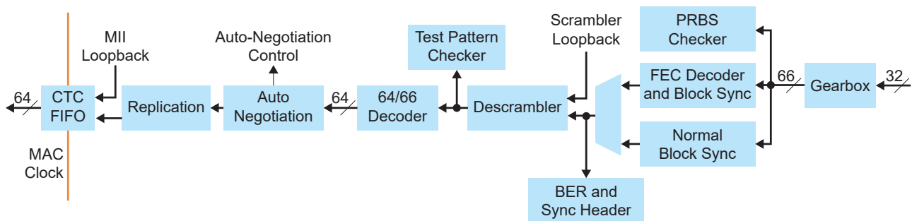
Figure 4: 10GBase-KR Receiver
