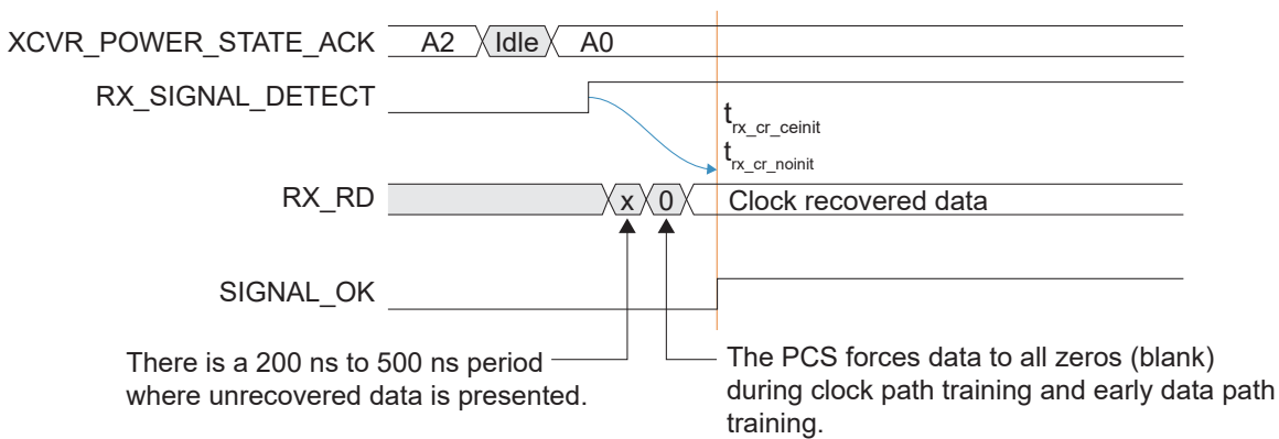
Figure 8: Asserting signal_ok
